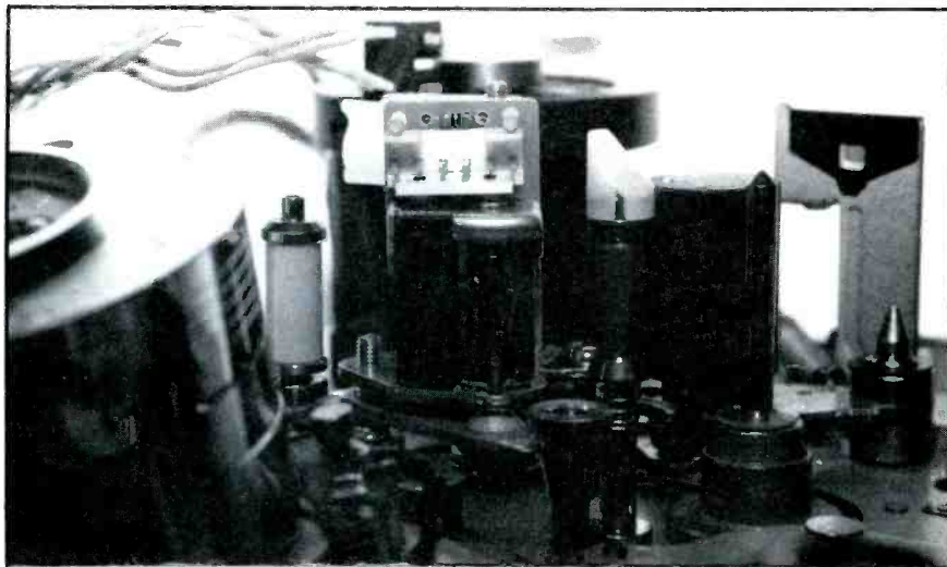
Proper adjustment of the tape transport system assures proper contact of the tape with the CTL/audio head, as shown here.
